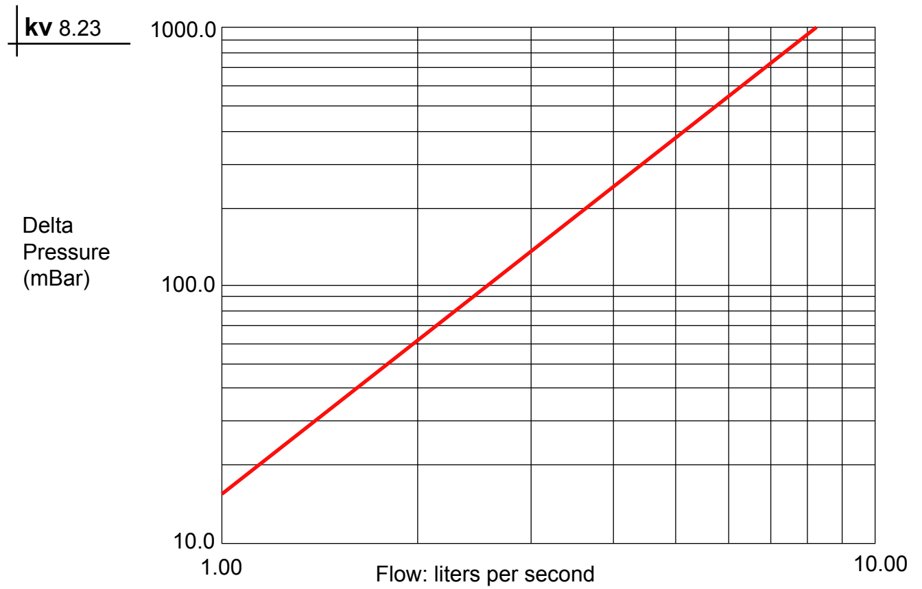
Diagram 990844/TA/2: test of loss of pressure due to flow rate of ELCLA4A Ø 1.1/2" magnetic scale preventer.
