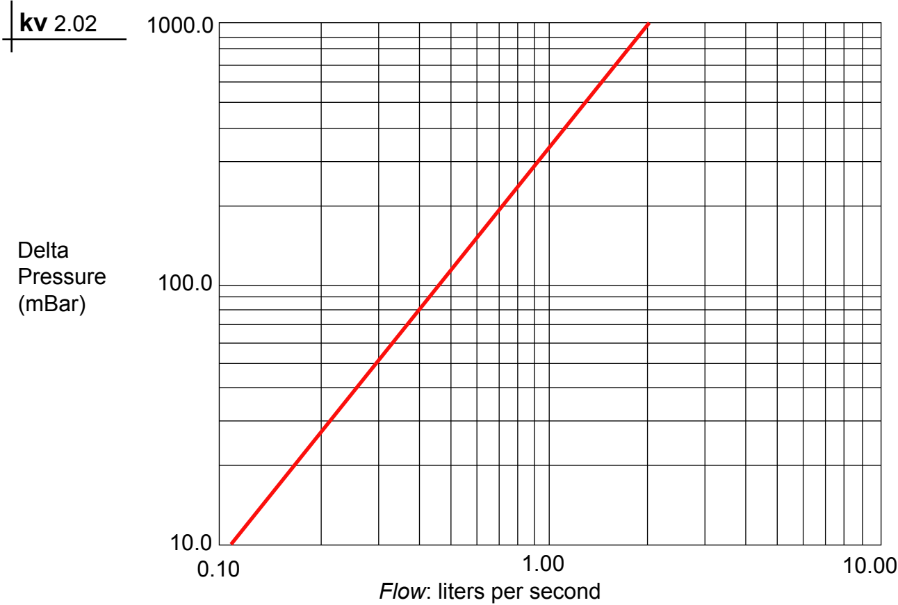
Diagram 981559/2: test of loss of pressure due to flow rate of ELCLA1 Ø 1/2" magnetic scale preventer.
