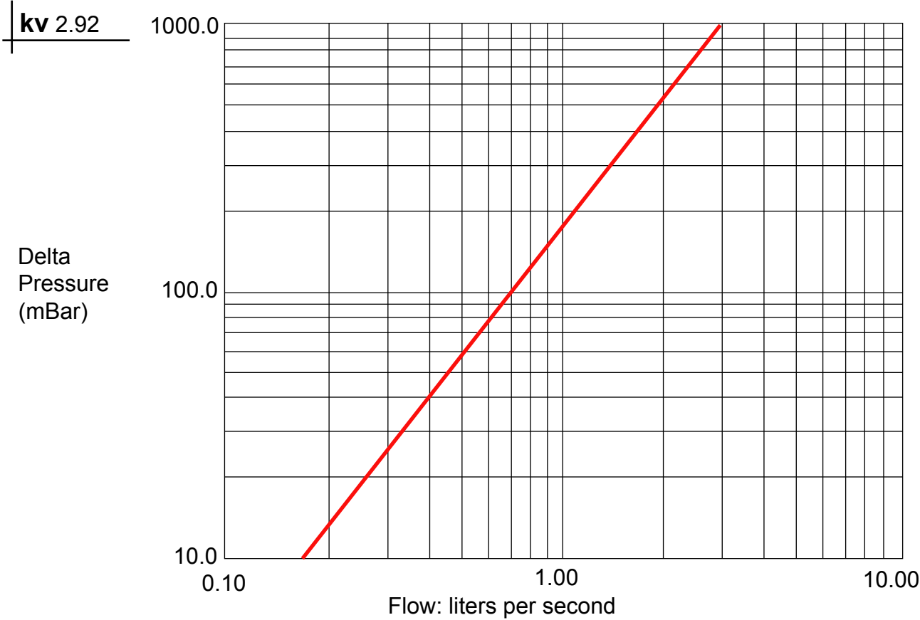
Diagram 981559/3: test of loss of pressure due to flow rate of ELCLA2 Ø 3/4" magnetic scale preventer.
