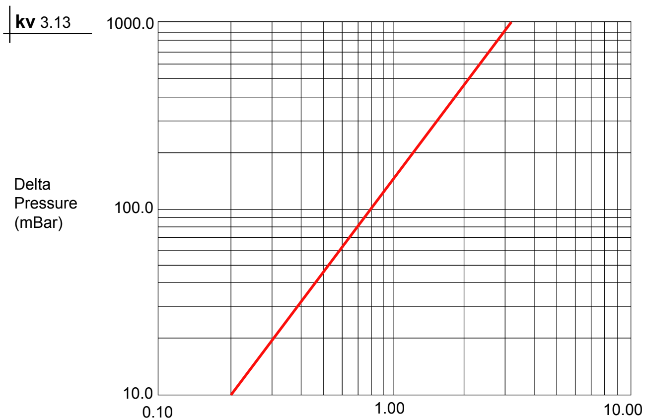
Diagram 981559/4: test of loss of pressure due to flow rate of ELCLA3 Ø 1" magnetic scale preventer.
