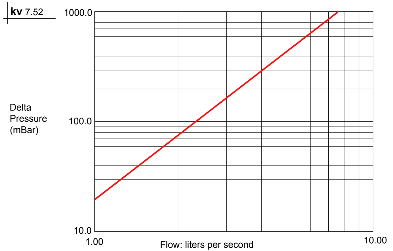
Diagram 990844/TA/1: test of loss of pressure due to flow rate of ELCLA4 Ø 1.1/4" magnetic scale preventer.
