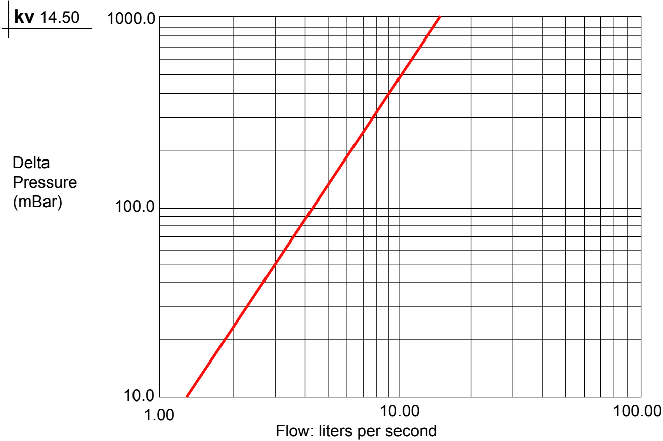
Diagram 990844/TA/3: test of loss of pressure due to flow rate of ELCLA5 Ø 2" magnetic scale preventer.
